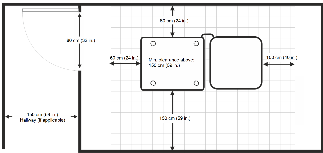
Figure 4 Printer floor plan (sample, not to scale)
