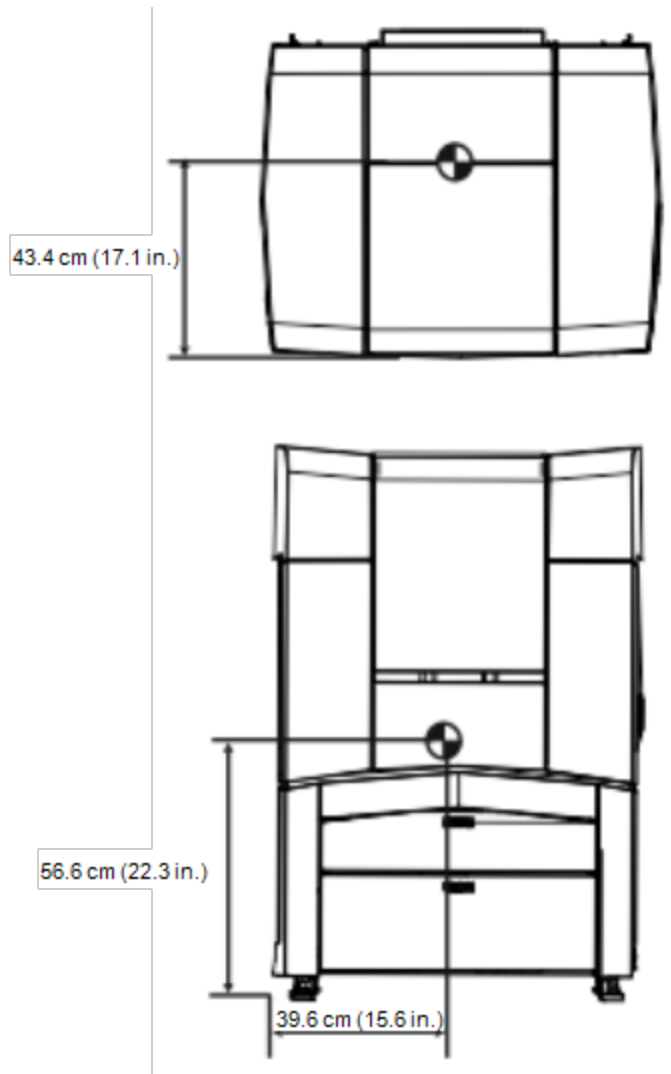
Figure 3 Printer center of gravity
