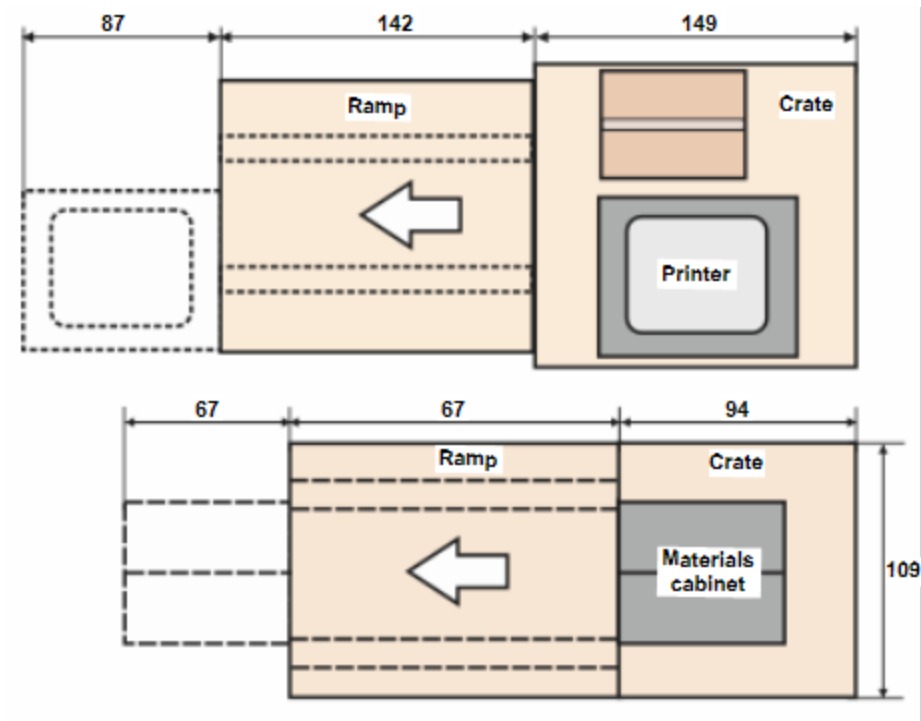
Figure 2 Unloading dimensions—top view
