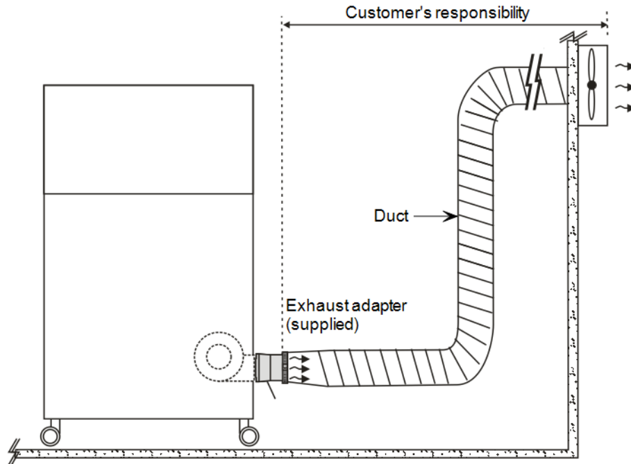
Figure 7 Printer exhaust system
